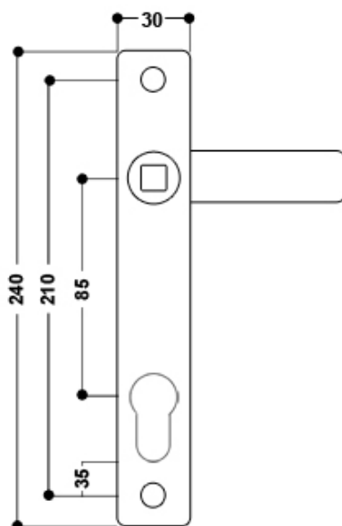
Suits UCEM mechanism.
